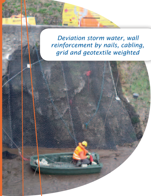
Nailed gravity flow and masonry
